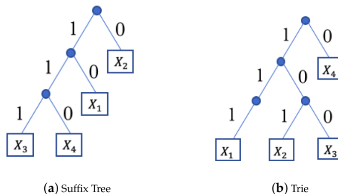
Figure 1. The suffix tree in (a) is built over the first four suffixes of string X = 101110\dots , and the trie in (b) is build over strings X_1 = 111\dots , X_2 = 101\dots , X_3 = 100 , and X_4 = 010\dots
